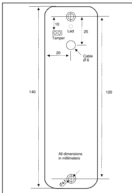
Access Slim housing
